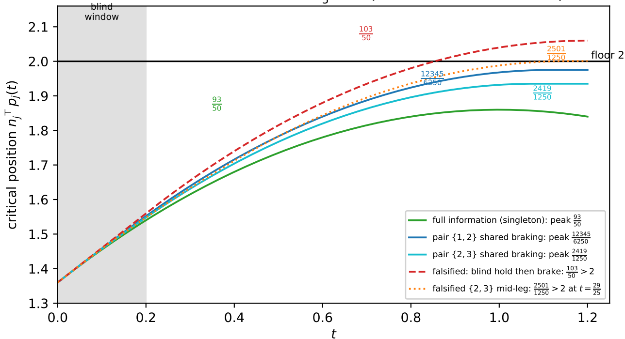
The three-branch instance at \tau = \frac{1}{5} : the policies and their exact peaks
